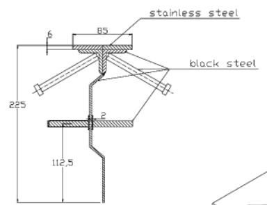
CONECTO SINUS 06NC85-5D h=225 stainless steel SECTION
