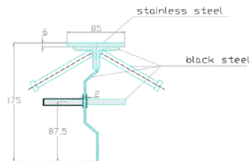
CONECTO SINUS 06NC85-5D h=175 stainless steel SECTION
