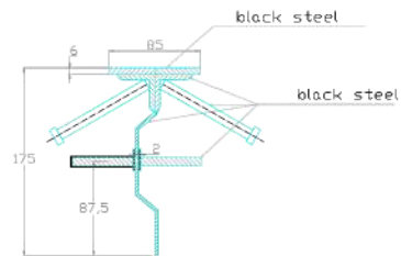
CONECTO SINUS 06NC85-5D h=175 black steel SECTION
