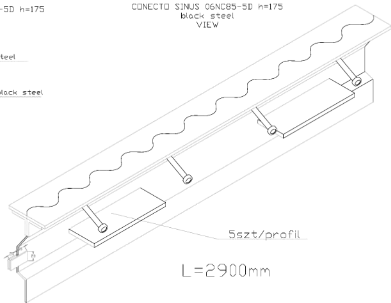
Expansion joint Conecto Sinus 06NC85-5D h=175 black steel
