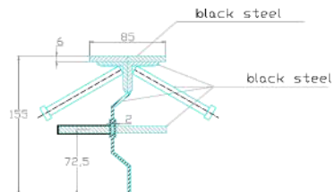
CONECTO SINUS 06NC85-5D h=155 black steel SECTION
